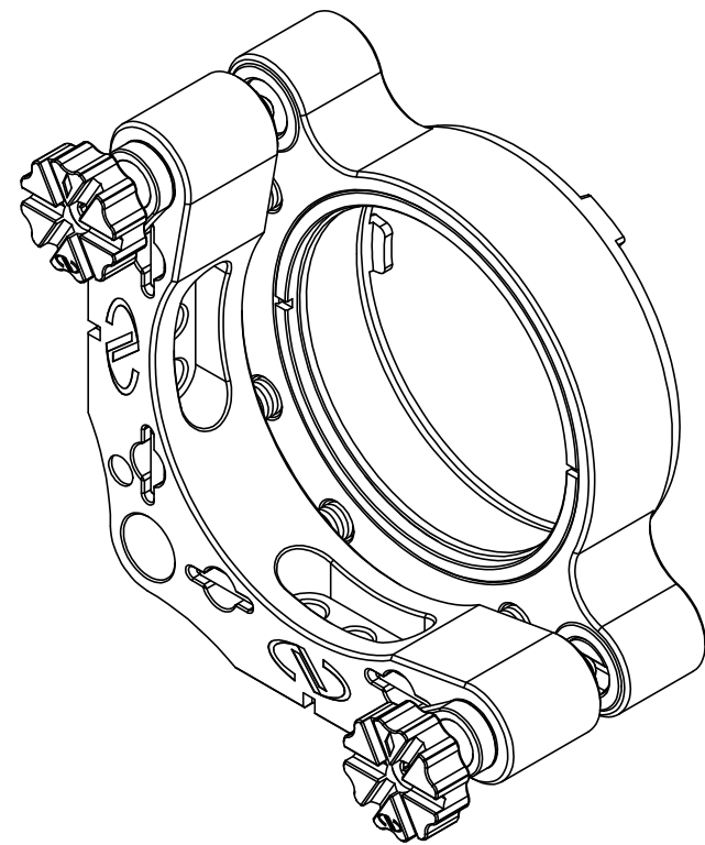
MODEL ST200T-R2K REAR LOAD, 2 KNOB ADJUSTORS
